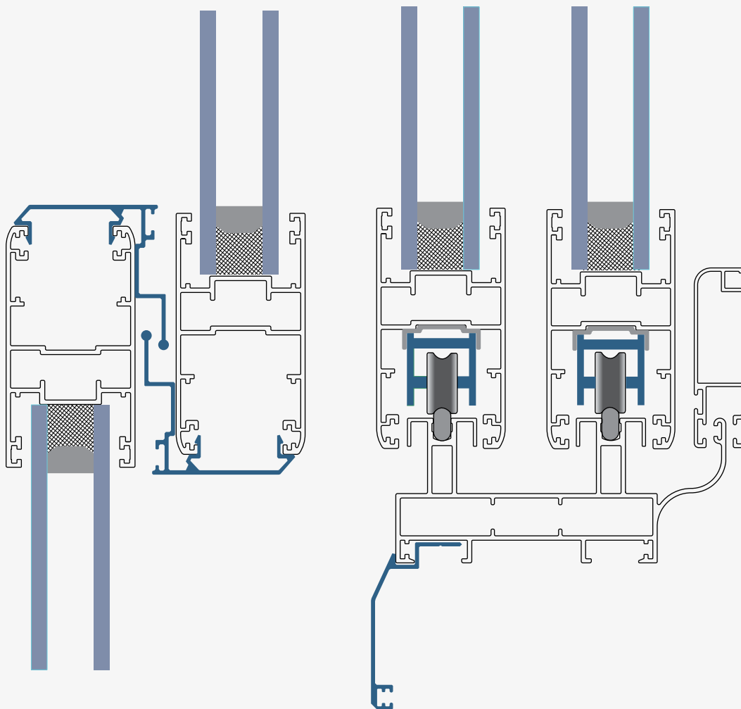
Section B
